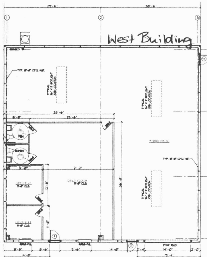
FLOOR PLAN
