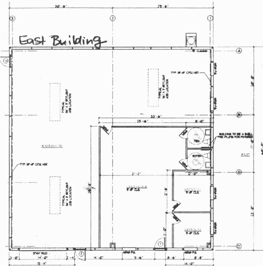
FLOOR PLAN
